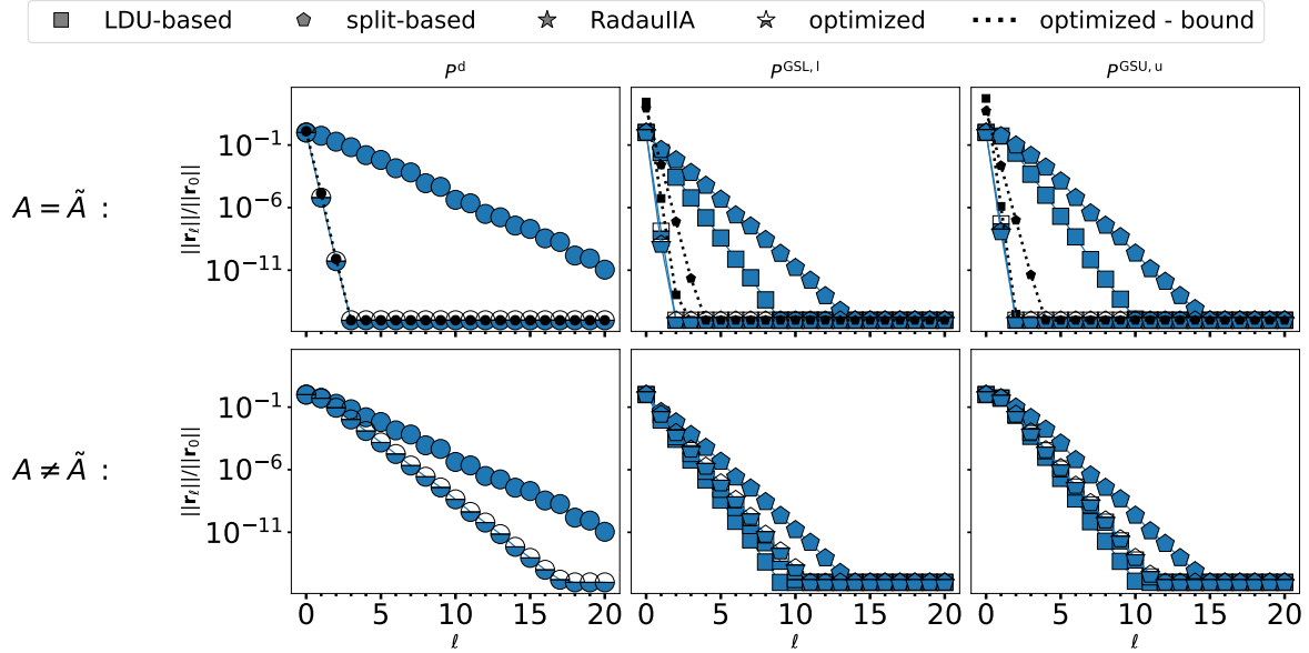
Figure 4: GMRES convergence (and bounds) for block preconditioners P^d (left column), P^{GSL,l} , P^l (middle column) and P^{GSU} , P^u (right column) for the two stage RadauIIA Butcher tableau (filled markers, same results as in Figure 2 and 3) and also the optimized setting considered above (half-filled markers). In the second row the optimization process changes only the matrix \tilde{A} used to construct the preconditioner (and not M ) in contrast to the first row where the optimized is used for construction of both the system matrix and the preconditioner (in this case we imposed A to be such that the resulting IRK method is at least of order two and is L -stable, the constraints can be found in [11, Section 7.3.4]). We used \omega = 10^{-5} , N = 100 and \tau = h^{2/p} as above.
