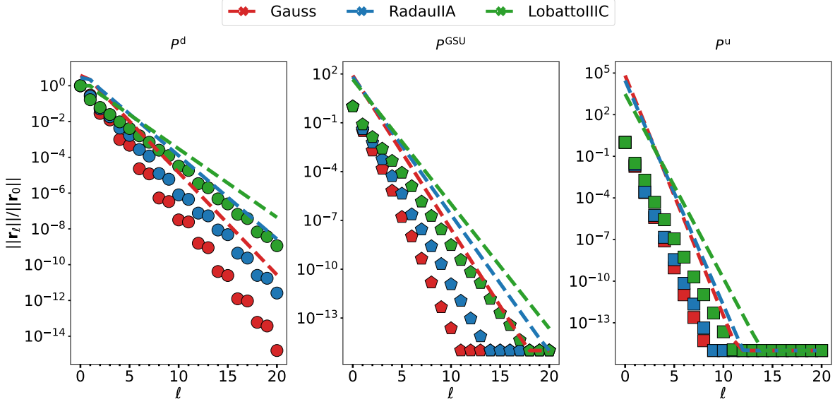
Figure 2: We show the GMRES performance together with the evaluated bound (10) for different preconditioners and Butcher tableaux. We set N = 100 , \tau = h^{2/p} ( p is the order of convergence of the IRK method; p_{\text{Gauss}} = 4, p_{\text{RadauIIA}} = 3, p_{\text{LobattoIIC}} = 2 ) and use a random right-hand side.
