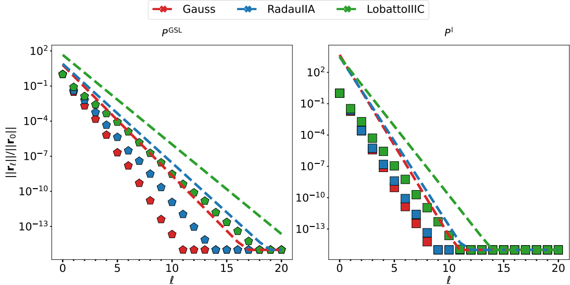
Figure 3: We show the GMRES performance together with the evaluated bound (10) for different preconditioners and Butcher tableaux. We set N = 100 , \tau = h^{2/p} ( p is the order of convergence of the IRK method; p_{\text{Gauss}} = 4, p_{\text{RadauIIA}} = 3, p_{\text{LobattoIIC}} = 2 ) and use a random right-hand side.
